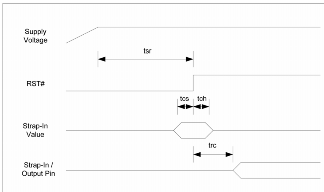
Figure 18. Reset Timing
